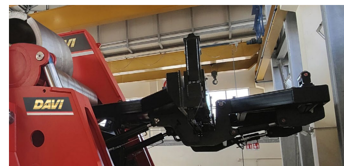
Side supports
